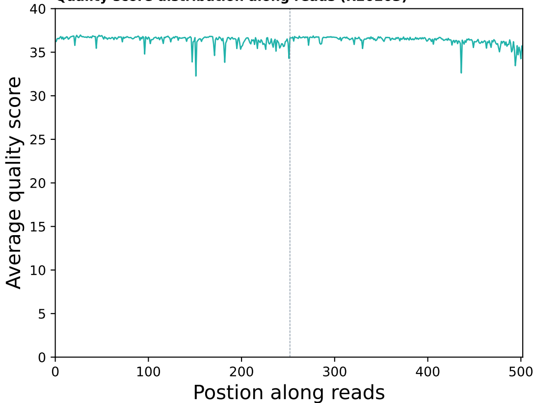
Quality score distribution along reads (R20203)
